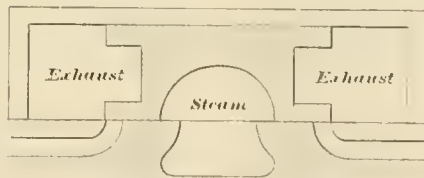
FIG. 4. D-VALVE—INSIDE ADMISSION.
